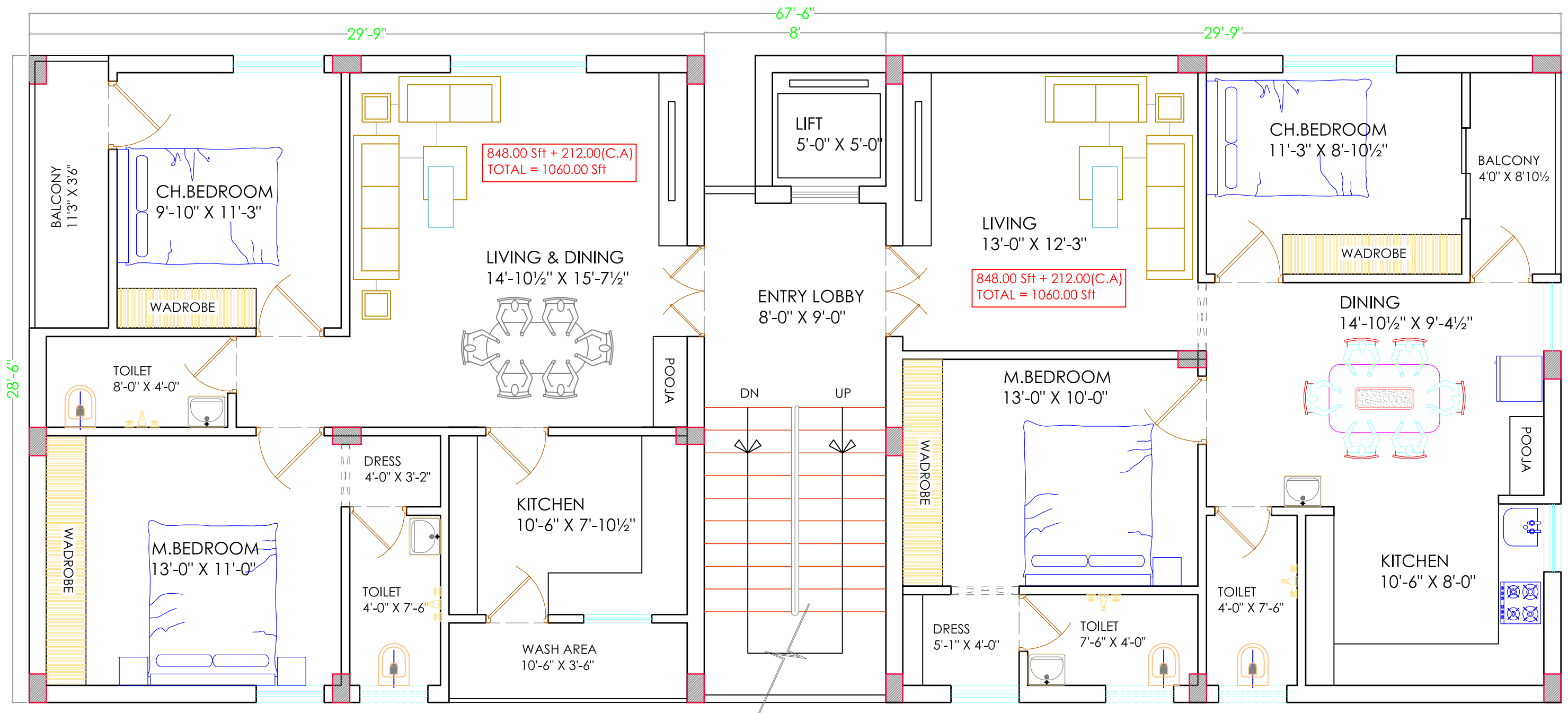
TYPICAL FLOOR PLAN SLAB AREA :- 1923.75 Sft
